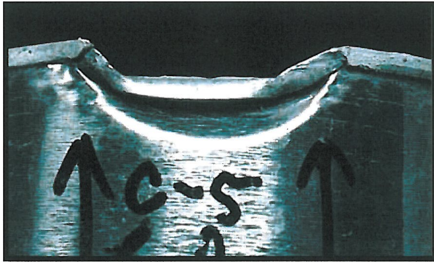
Photo 5: Severe double seam dent plate fracture.
