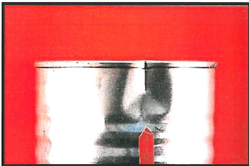
Photo 4: Plate fracture in double seam or can body. Note position of red pointer.
